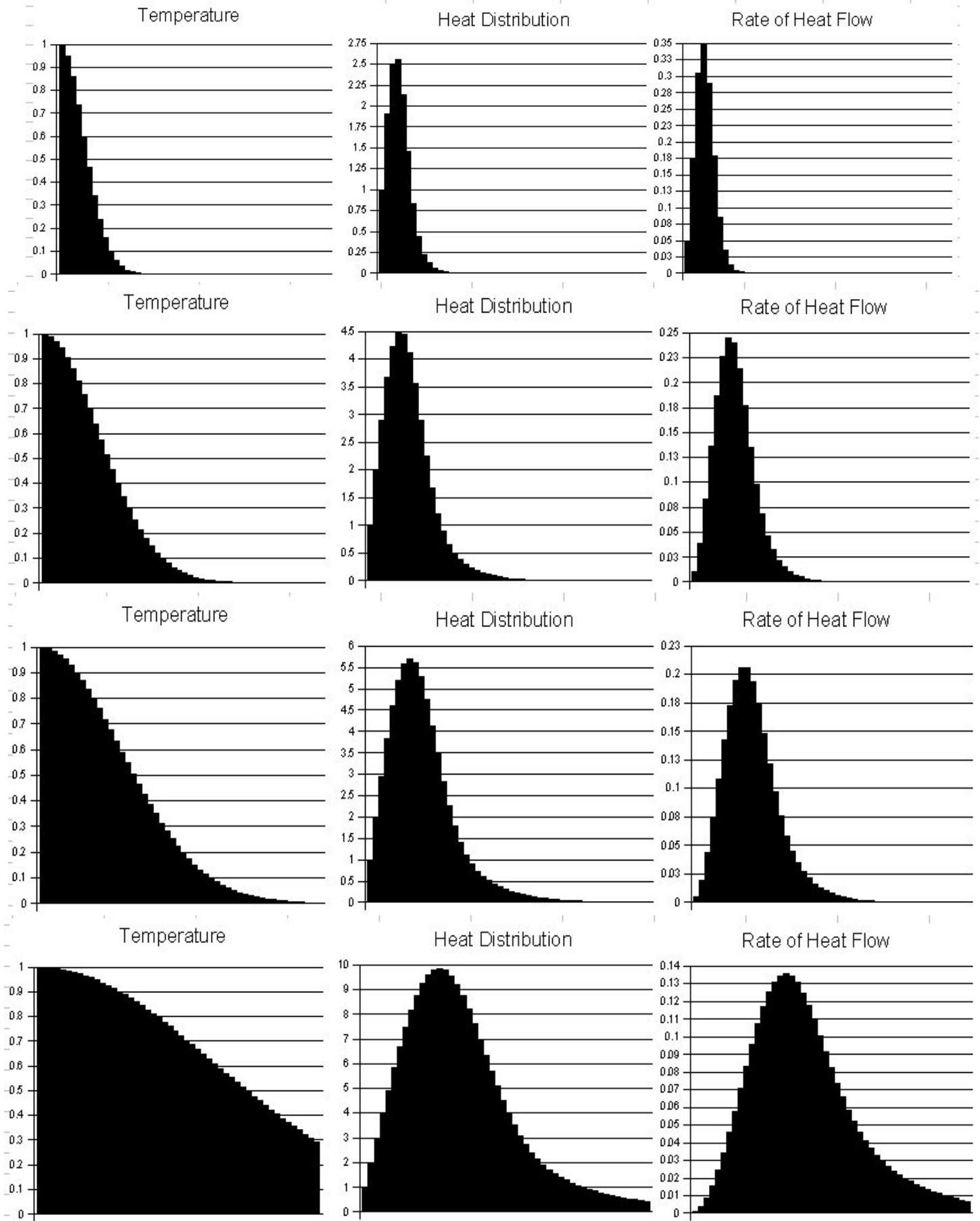
Program AE-1 was used to plot the temperature, heat distribution and rate of heat flow from the center to the periphery for heat injection at a rate that maintains the borehole temperature at a constant value (various times).
